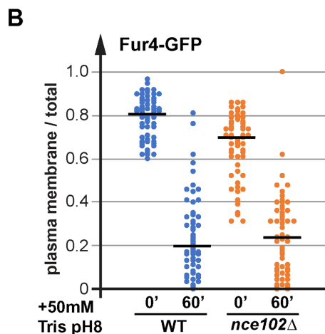
FIGURE 8: Eisosome mutations do not impair endocytosis or cell integrity. (A) Wild-type and mutant cells were grown in SD_{comp} + 1 M sorbitol. The cells of the midlog yeast cultures were moved into SD_{comp} pH 4 medium and after 10 min the cells were stained with PI and analyzed by flow cytometry. (B) Microscopy pictures of Fur4-GFP expressing cells (WT, SEY6210 pJK19; nce102Δ , AMY41 pJK19) in the presence or absence of 50 mM Tris, pH 8, were quantified by determining the signal at the plasma membrane of Fur4 relative to the total signal. The graph shows the result of ~50 cells for each strain and condition. The black line indicates the median of the data set.
